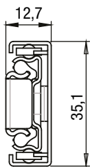
Guide a sfere e guide a rullo | Guide personalizzate Ball-bearing slides and roller slides | Customized Slides
