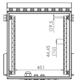
INSIDE VIEW
